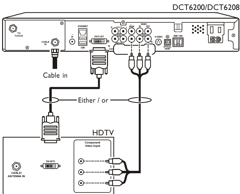
DVI connection
